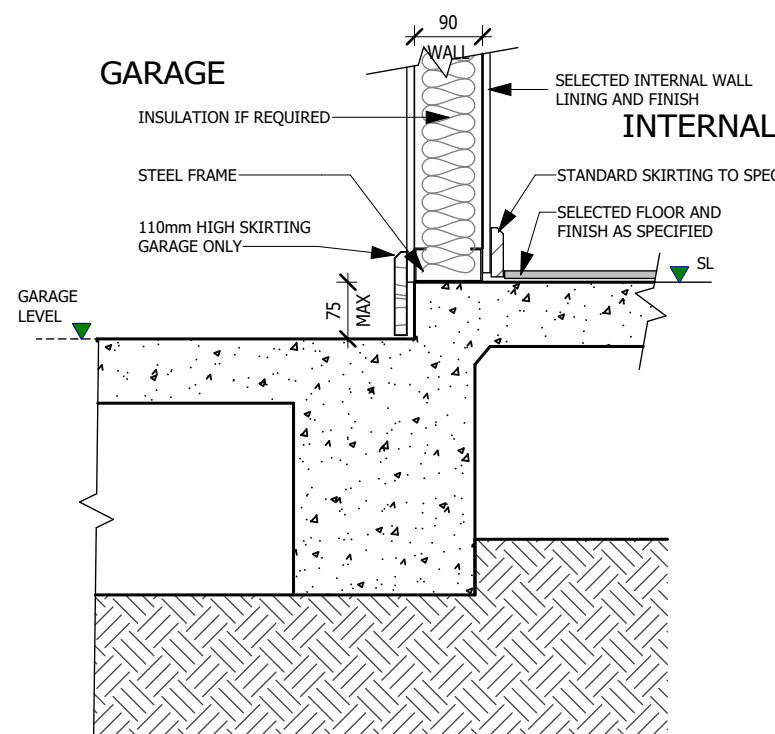
4 INTERNA GARAGE STEP - 75MM STEP ONLY SCALE: 1 : 10
