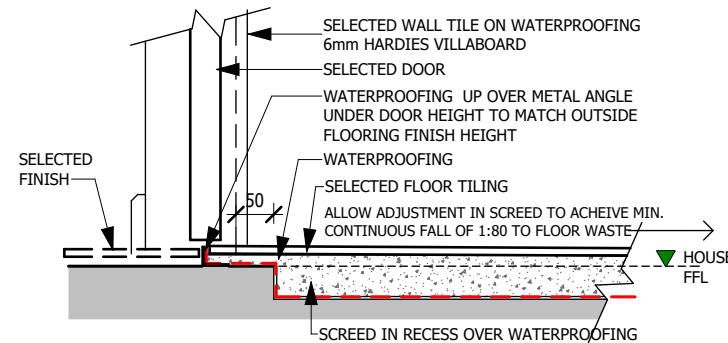
1 WET AREA DOOR THRESHOLD
