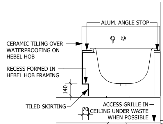
2 BATH WITH WINDOW DETAIL
