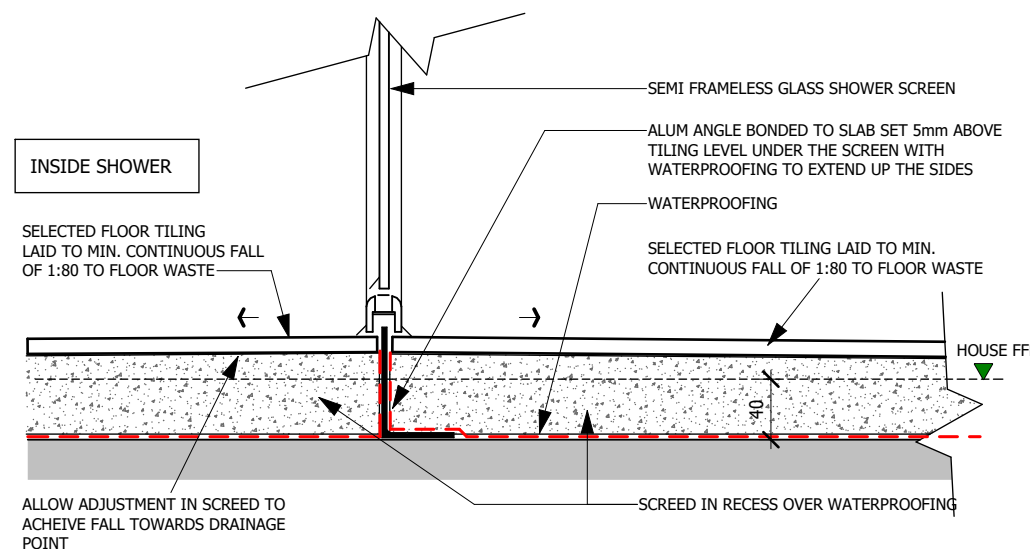
3 SEMI FRAMELESS SHOWER SCREEN DETAIL
