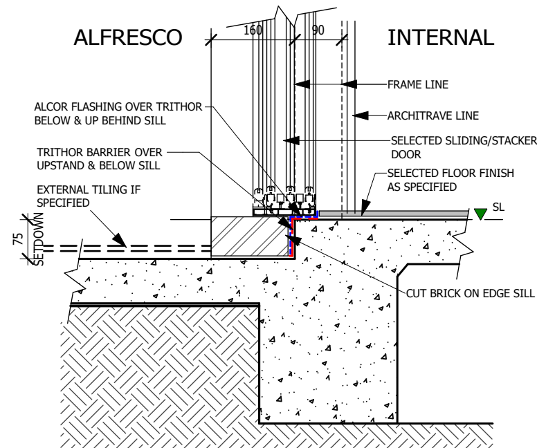
3 ALFRESCO DOOR - BRICK VENEER SCALE: 1 : 10
