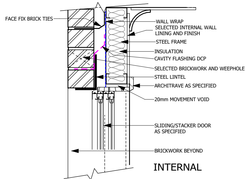
3 SLIDING DOOR HEAD - BV1 SCALE: 1 : 10
