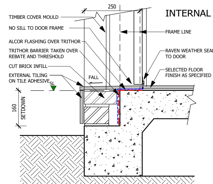
4 LAUNDRY TIMBER DOOR SCALE: 1 : 10
