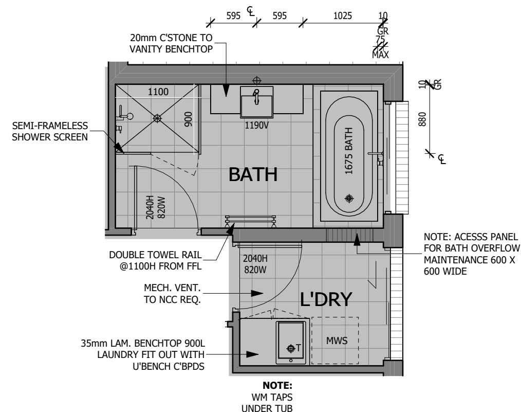
MAIN BATH & LAUNDRY
